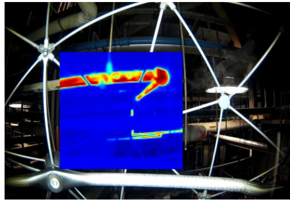
Steam leak view from UAV thermal camera
