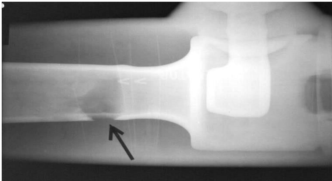
Radiograph of Ruptured Spray Nozzle Assembly
